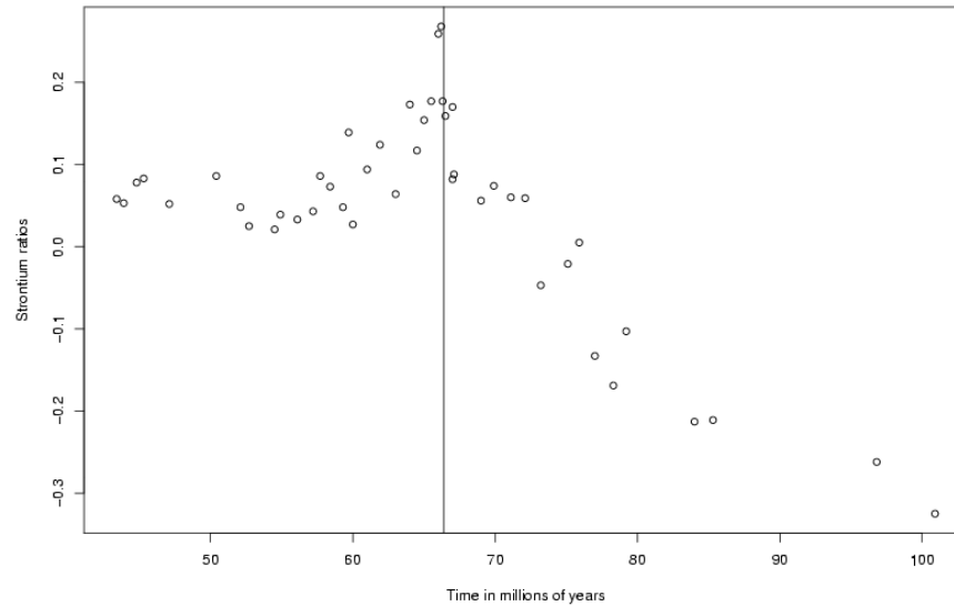
Figure 9.1: ^{87}\delta\text{Sr} data.
