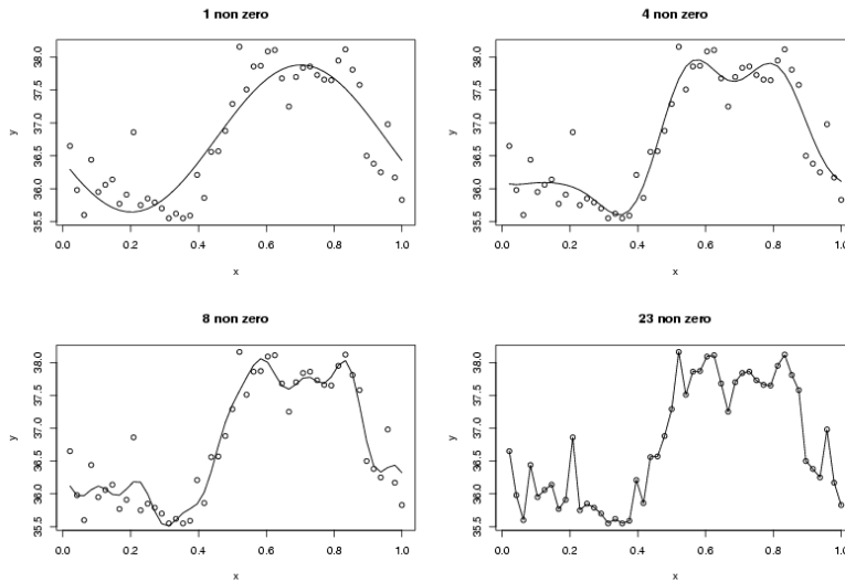
Figure 9.8: Fitted curves obtained when using shrinkage coefficients of the form w = (1, 1, \dots, 1, 0, \dots, 0) , with 2m + 1 the number of 1s used.
