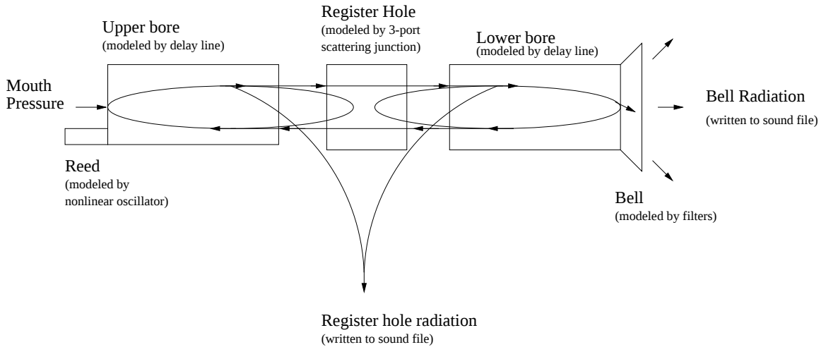
Figure 2.3: Clarinet modeled as a five-part structure.
