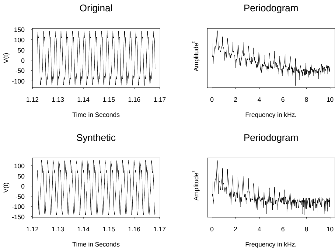
Figure 5.1: Comparison of original and synthetic clarinet signals.
