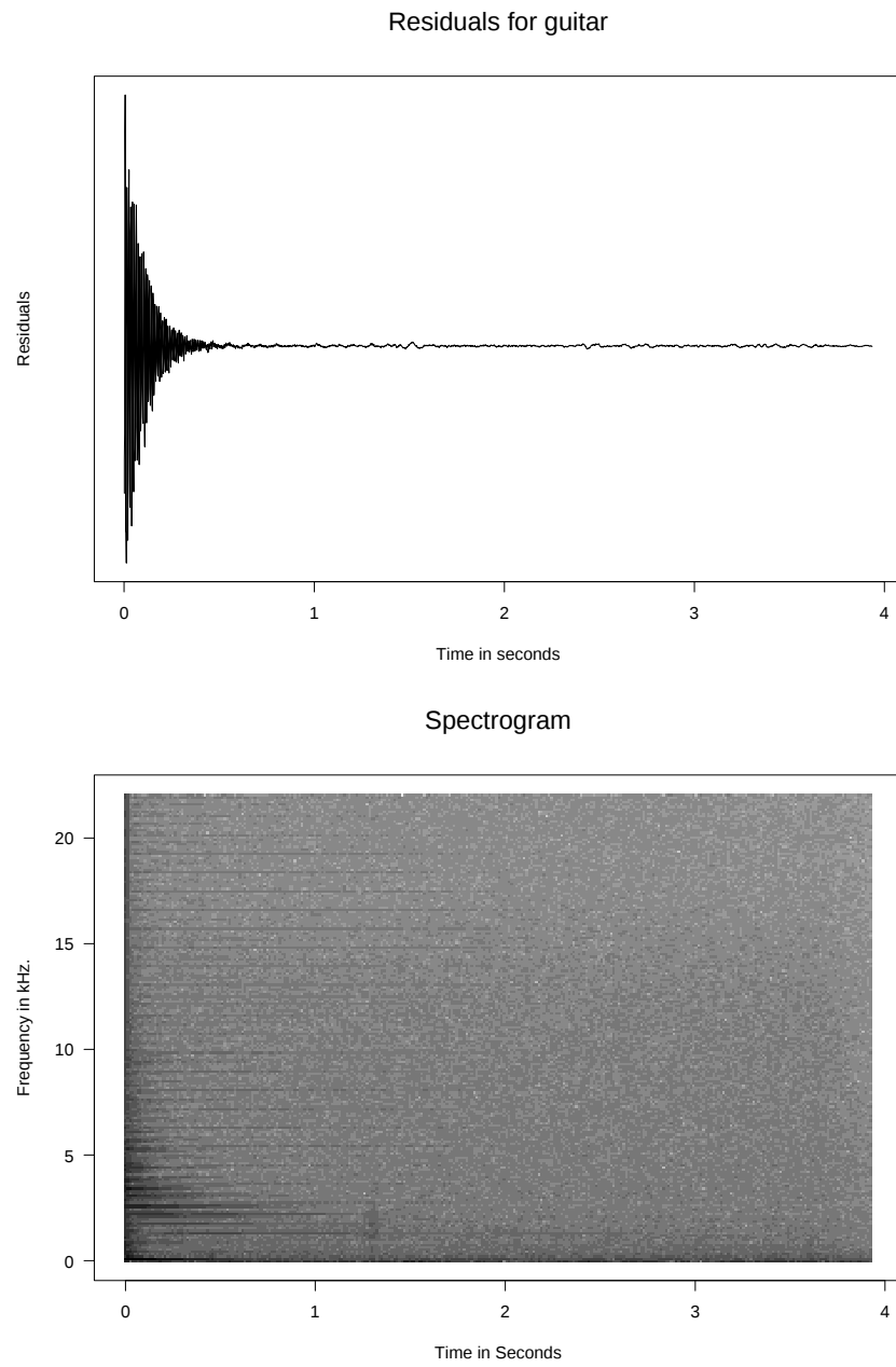
Figure 6.14: Global residuals and spectrogram for the sound signal of a guitar playing D3.
