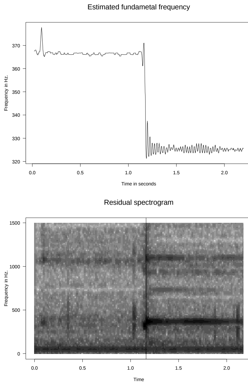
Figure 6.27: Frequency estimate for the sound signal of the pipe organ sound using one fundamental model and spectrogram for the residuals.
