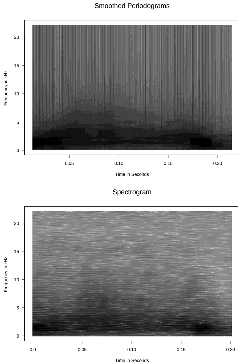
Figure 6.12: Smoothed periodograms of local residual for each sampled time and spectrogram of the global residuals for the sound signal of a trumpet playing D3.
