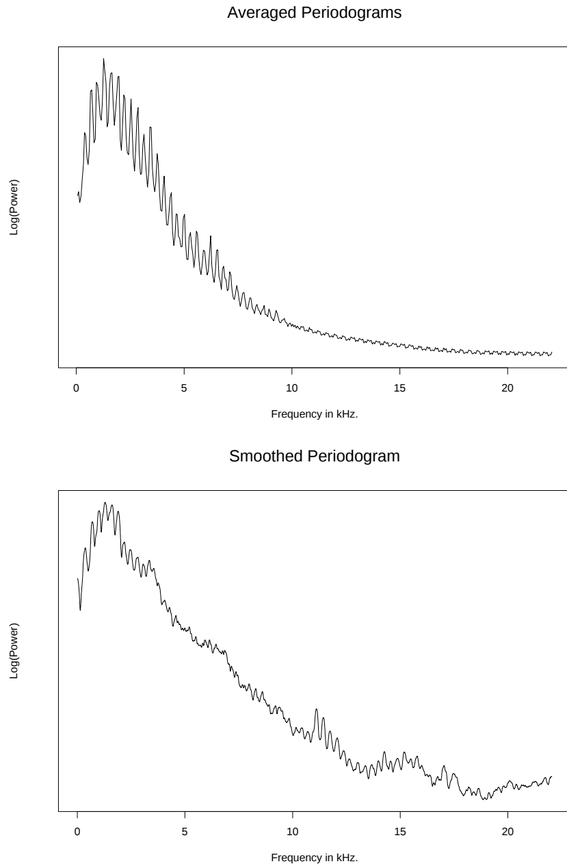
Figure 6.11: Averaged periodogram of the local residuals and smoothed periodogram of the global residuals for the sound signal of a trumpet playing D \sharp 3.
