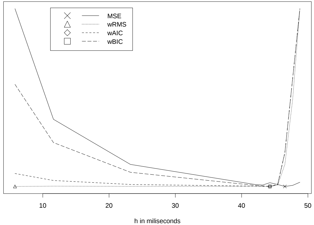
Figure 5.4: Comparison of weighted RMS, AIC and BIC for a change of pitch.
